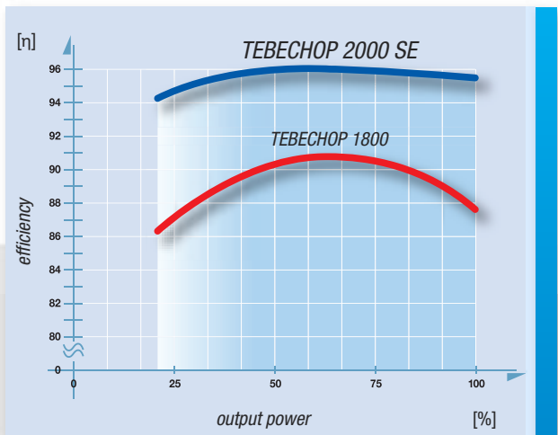
Fig. 2: Efficiency and output power
